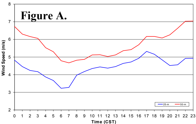
Diurnal Wind Speed Pattern
